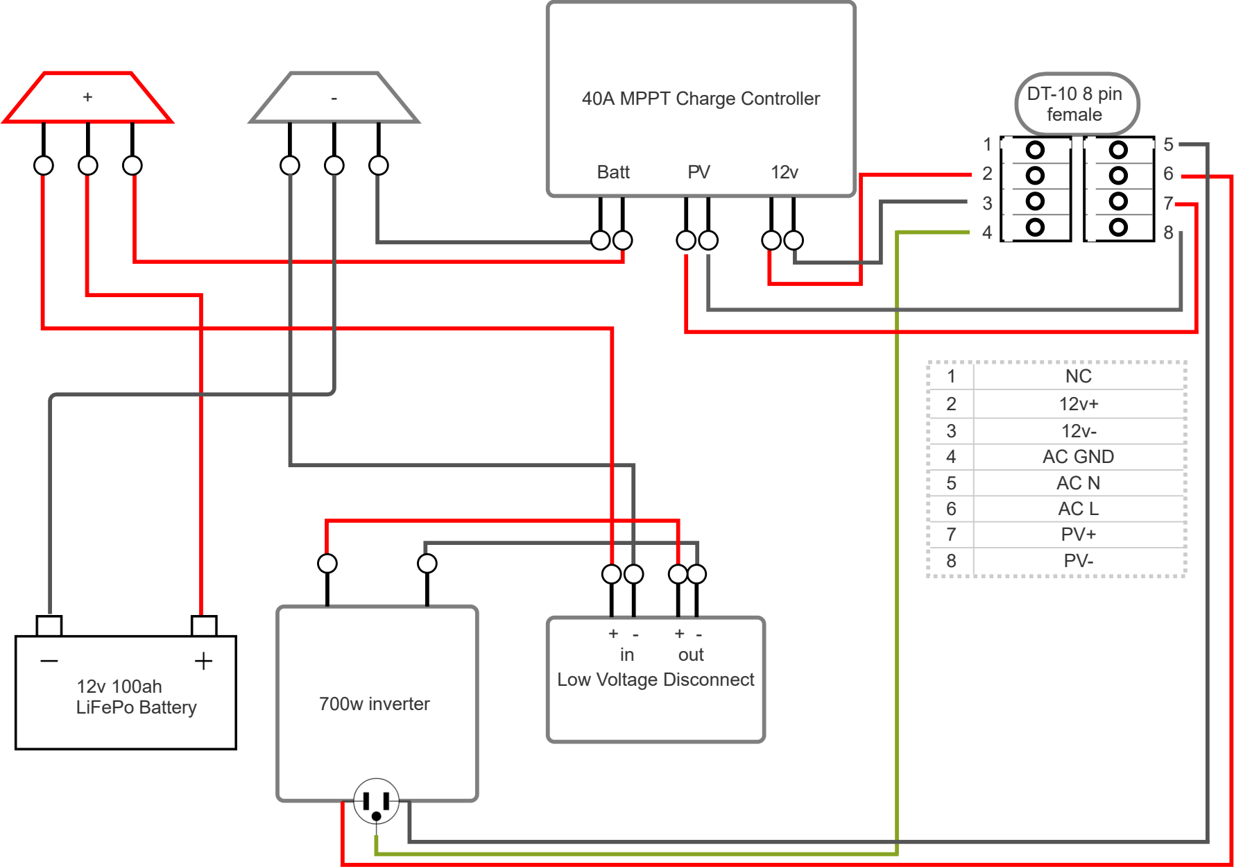
Battery Box WIRING DIAGRAM v1.1
